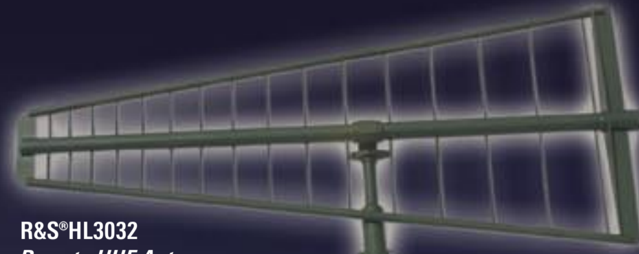
R&S®HL3032 Remote UHF Antenna, 225 MHz to 400 MHz, log-periodic
